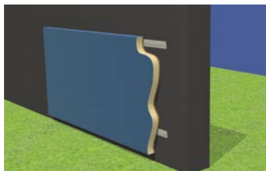
Z-clip attachment to a solid wall or structure
