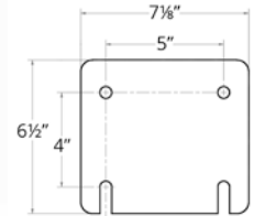
Mounting Plate
