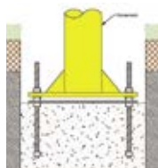
Leveling Plate
