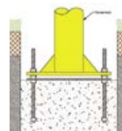
Leveling Plate
